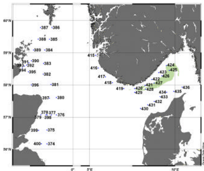
Fig. 2. Map of the primary and secondary transect stations sampled for HAB organisms and their toxins in association with physical and biophysical parameters in the coastal North Sea.
