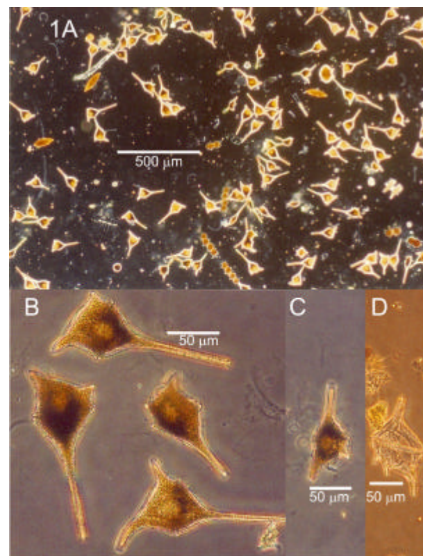
Fig. 1. A) Ceratium balechii , dark field at 40x, 1 ml sample. B) Four cells of different size. C) Small cell. D) Anomalous specimen with three antapical horns. B-D) Phase contrast, 200x.
