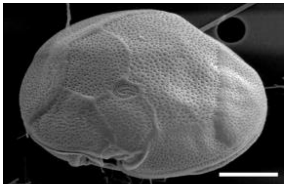
Fig. 2. SEM picture of Gambierdiscus sp. from the Canary Islands (scale bar: 20 μm).
