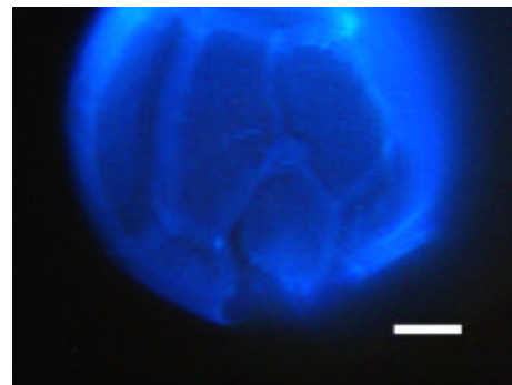
Fig. 5. Calcofluor-stained Gambierdiscus sp. cell from Crete showing Po and 1' plate (scale bar: 10 \mu m).
