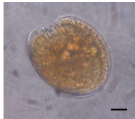
Fig. 3. Live Gambierdiscus sp. cell from Crete in apical view (scale bar: 15 μm).
