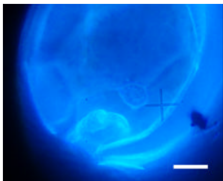
Fig. 6. Calcofluor-stained Gambierdiscus sp. cell from Crete showing Po and 1' plate (scale bar: 10 \mu m).
