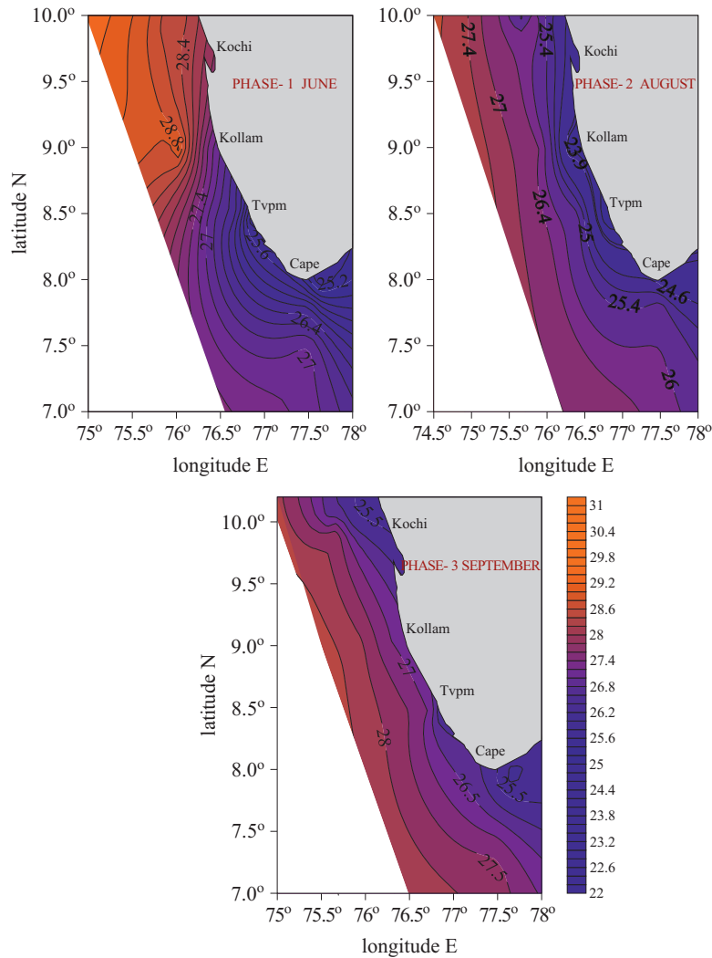
Figure 2. Variations in SST [°C] during different phases of upwelling along the SEAS during the summer monsoon of 2009
