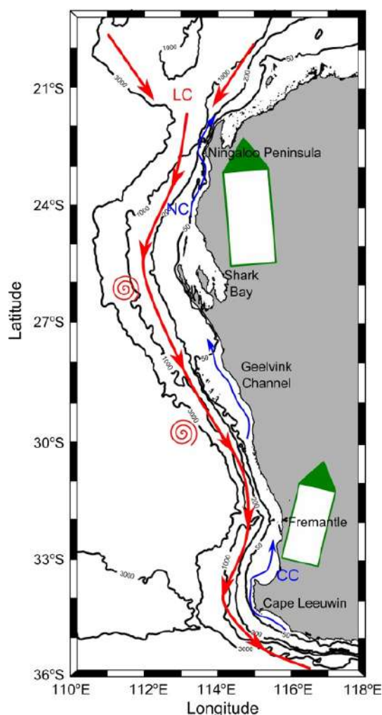
Figure 21. Map of the Western Australian coast with thin black contours showing the 50, 200, 1000, and 3000 m isobaths. Green arrows represent mean surface winds; red arrows indicate the Leeuwin Current; red schematic vortices indicate mesoscale eddies, and blue arrows indicate the Capes and Ningaloo currents (from Rossi et al., 2013b).
