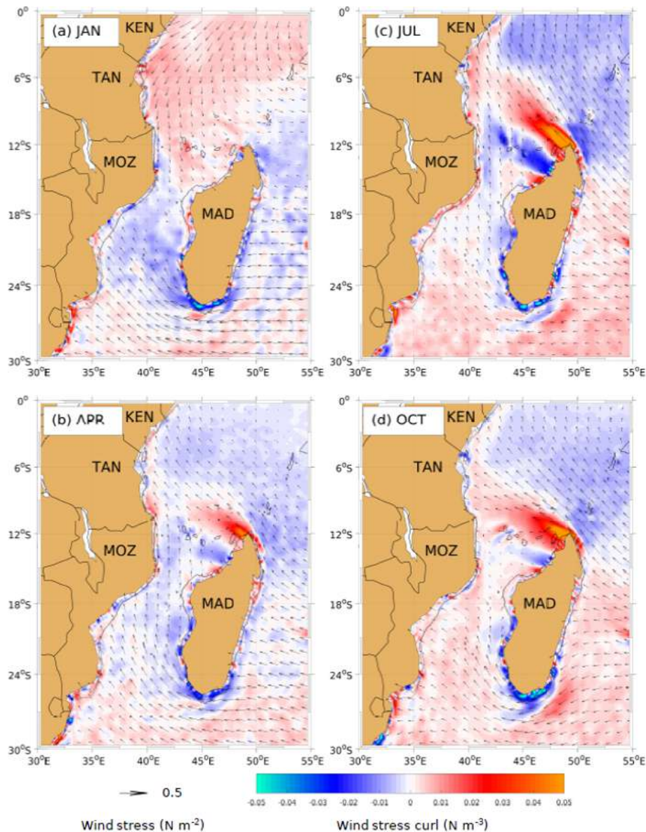
Figure 8. Climatological monthly means of wind stress (vectors) and wind stress curl (shading) during different seasons. Austral summer ( a , JAN), autumn ( b , APR), winter ( c , JUL) and spring ( d , OCT). Negative (blue) and positive (red) wind stress curl depicts favourable upwelling and downwelling areas, respectively. The data were extracted from the Scatterometer Climatology of Ocean Winds (SCOW), described by Risien and Chelton (2008); mapped globally with a spatial grid resolution of 1/4^\circ \times 1/4^\circ ; estimated from a 10-year period, ranging between September 1999 and August 2009; and measured by QuikSCAT.
