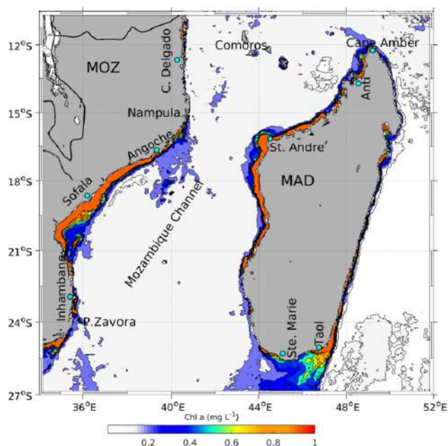
Figure 10. Monthly mean chlorophyll a concentration for February 2003, derived from the Moderate Resolution Imaging Spectroradiometer (MODIS) aboard the Aqua satellite ( https://oceancolor.gsfc.nasa.gov/data/aqua/ , last access: 5 November 2021). Intermediate values beyond the continental shelf edge highlight areas of elevated productivity off the Mozambique and Madagascar coasts that are primarily upwelling-driven. Abbreviations are Ponta Zavora (P. Zavora), Cabo Delgado (C. Delgado), Taolagnano (Taol), and Antsiranana (Anti).
