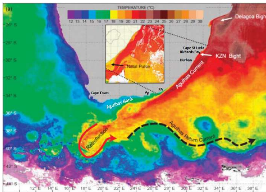
Figure 2. SST image highlighting the Agulhas Current flowing along the east coast of South Africa. PE is Port Elizabeth; PA is Port Alfred. Insert highlights a southwestward-propagating Natal pulse (a singular meander in the trajectory) which has a cold core. The shelf on the east coast is narrow with a steep continental slope. Exceptions are the KwaZulu-Natal (KZN) Bight and the Agulhas Bank.
