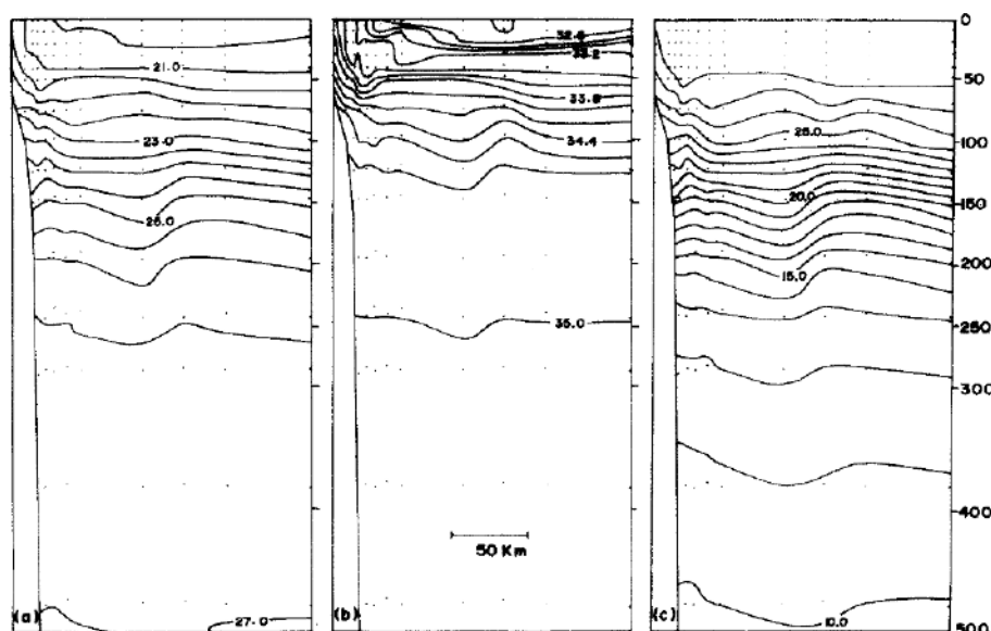
Figure 18. Hydrography along a section (normal to the coast) which lies approximately midway ( \sim 15^\circ \text{N} ) along the east coast of India. (a) Potential density ( \text{g cm}^{-3} ); (b) salinity (ppt); (c) temperature ( ^\circ \text{C} ). The scale shown in (b) also applies to (a, c) (from Shetye et al., 1991).
